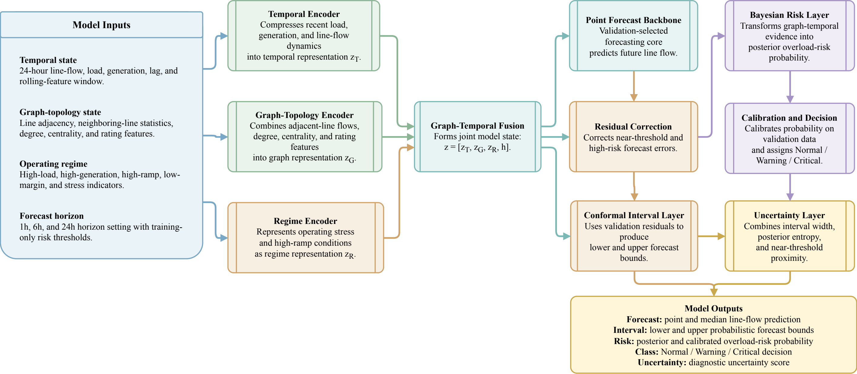
Component view of the Bayesian Temporal Graph Probabilistic Risk Forecaster
